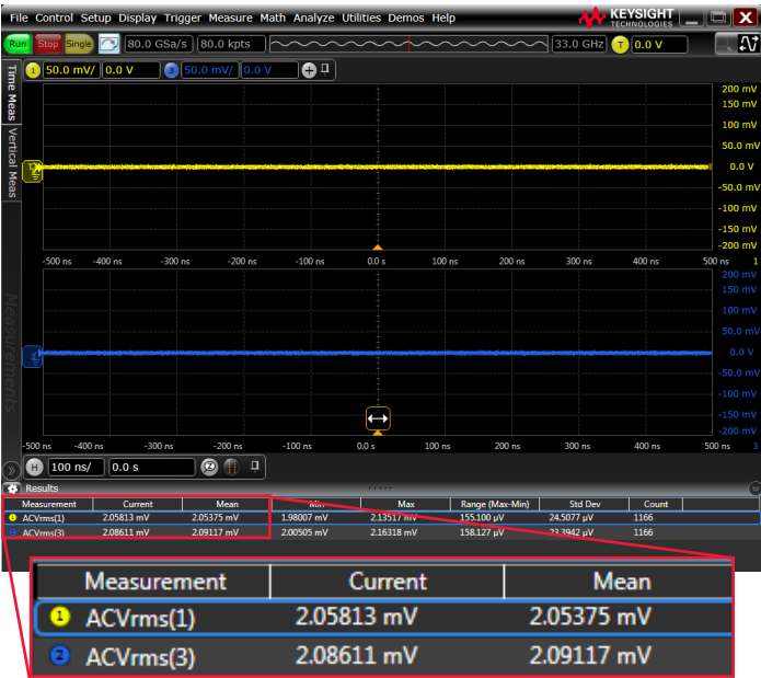
Ultra-low noise at 33-GHz full bandwidth (2.10 mV at 50 mV/div).
