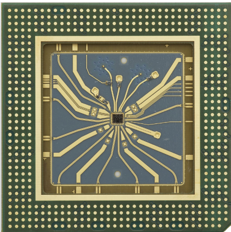
Keysight uses Indium Phosphide process to produce a 12 ps edge step response, ideal for characterizing cable and probe frequency response.
