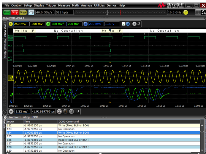
DDR3 protocol decode and write command trigger.
