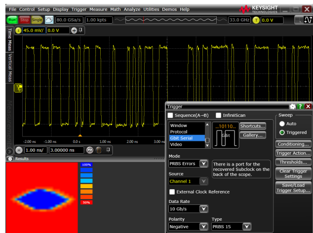
PRBS error detector triggers on a bit error in the PRBS-15 signal. An eye view plot (bottom left) is provided to show the quality of the signal received by the hardware serial trigger. The hardware serial trigger works when there is enough eye opening (blue area) to discern the bit value.
