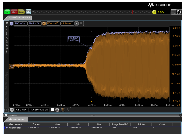
Envelope detection of signal burst.
