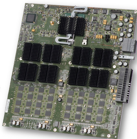
Acquisition board.
