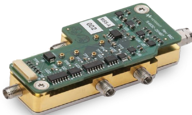
RealEdge technology blocks enable 63-GHz real-time bandwidth.
