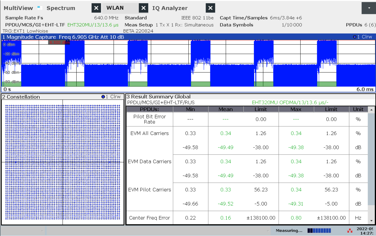
Measured EVM for an IEEE 802.11be signal with 320 MHz bandwidth
