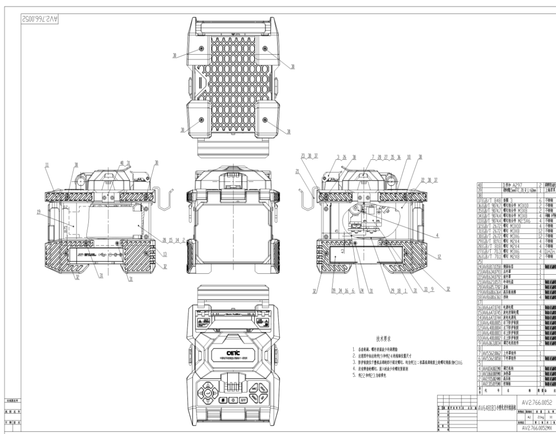
Fig.3 Overall appearance of instrument
