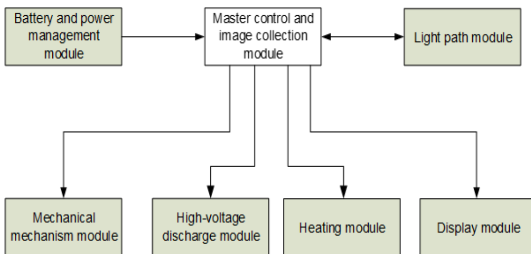
Fig.2 Block diagram of whole machine
