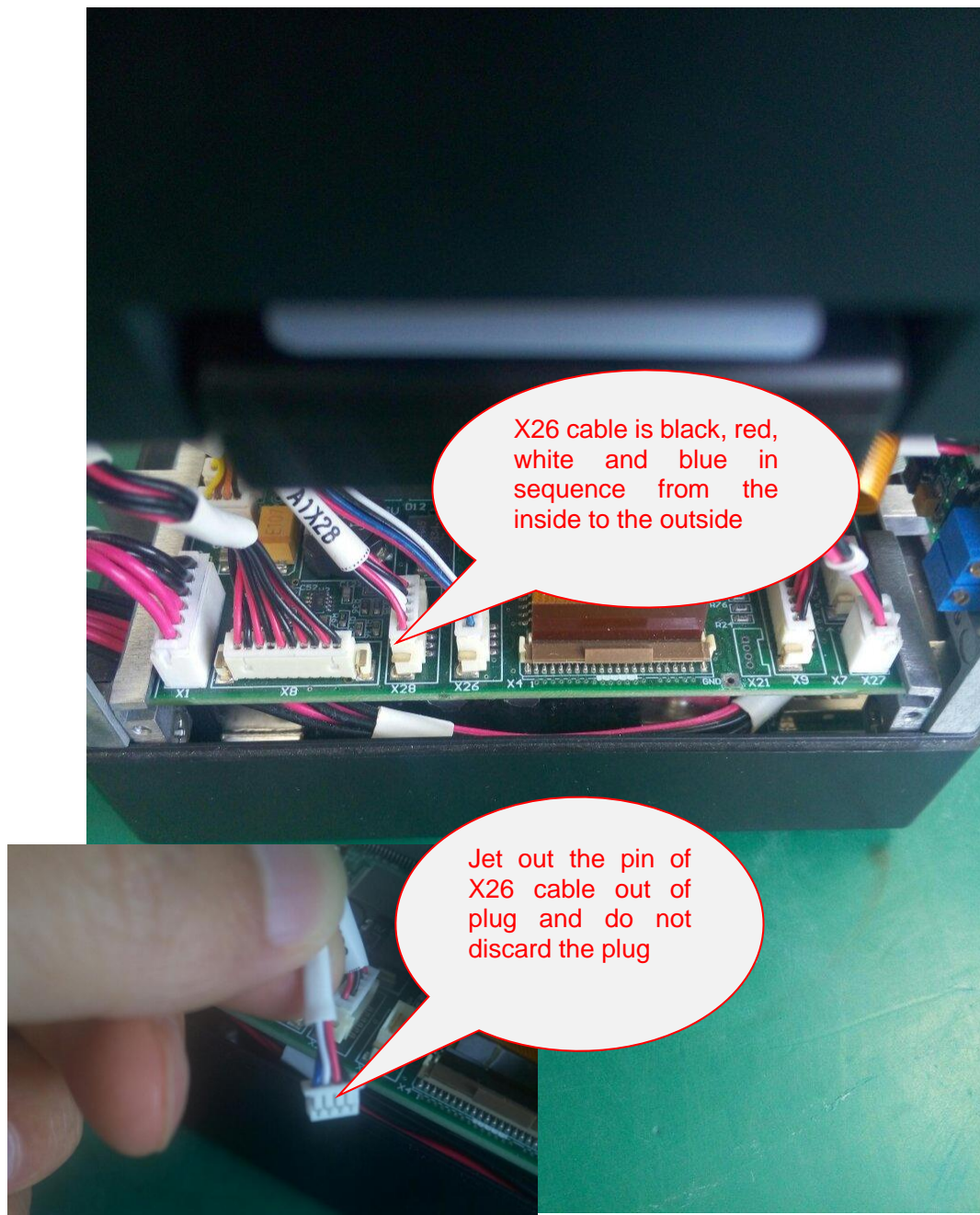
Fig.12 X26 cable
