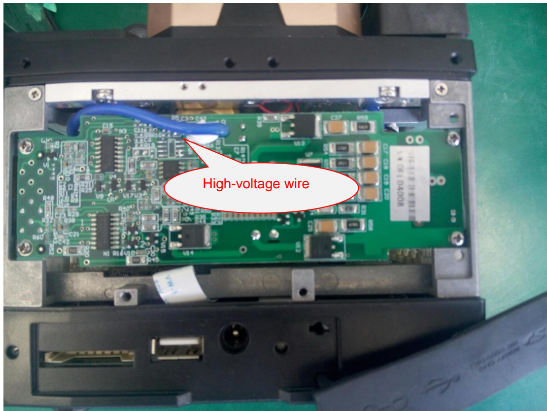
Fig.17 High-voltage board
