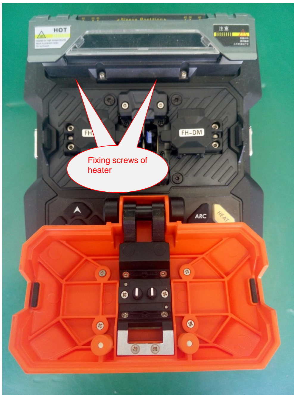
Fig.15 Heater
