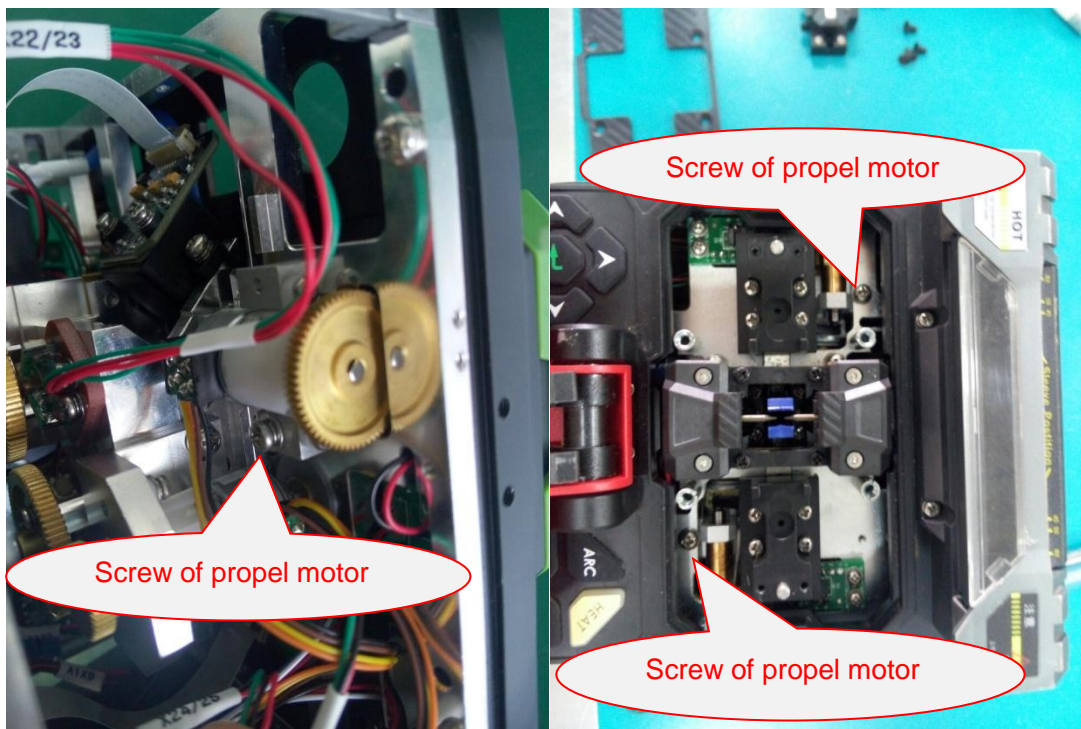
Fig. 6 Positions of propel motor screws
