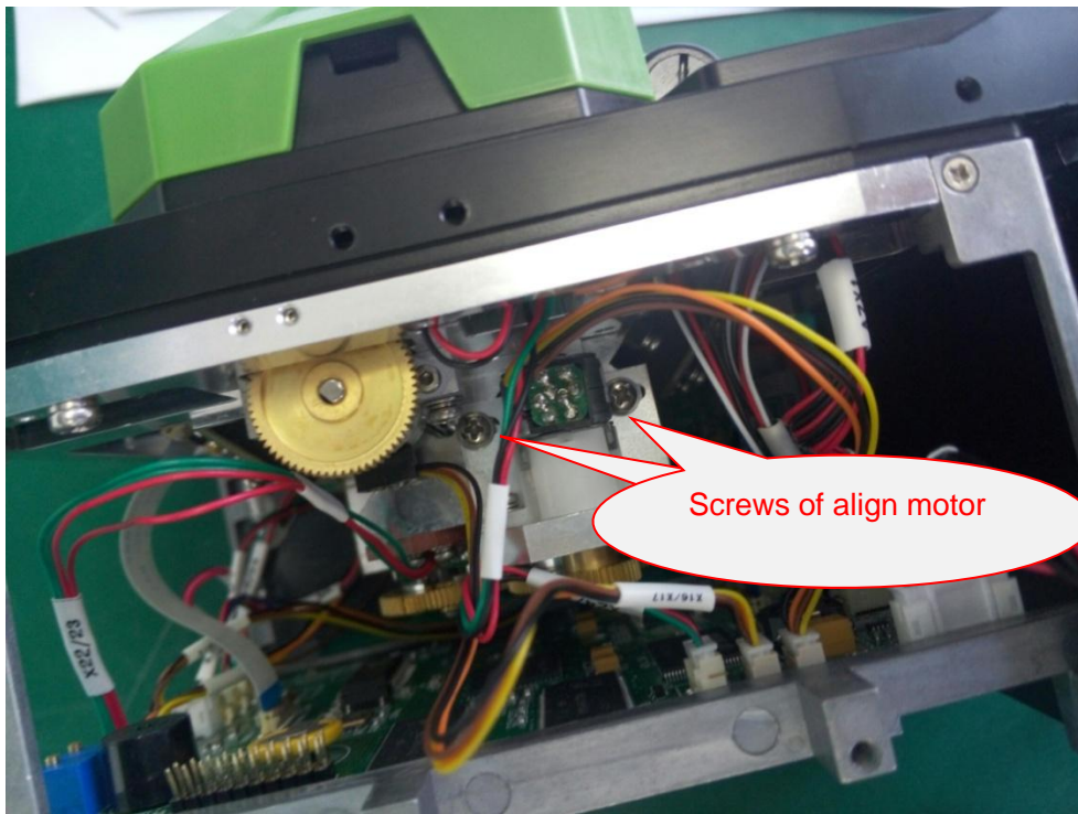
Fig.8 Align motor
