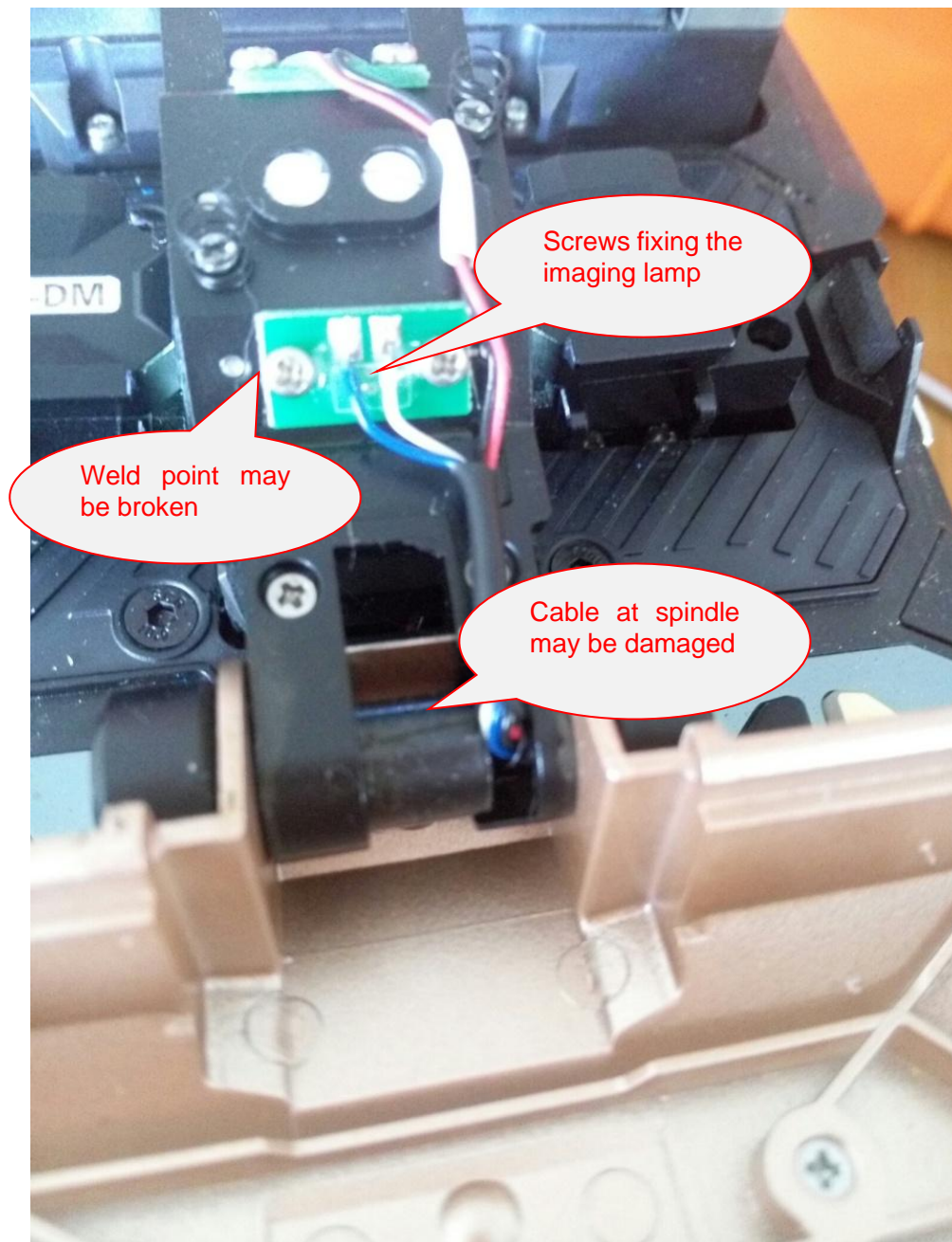
Fig.11 Imaging lamp
