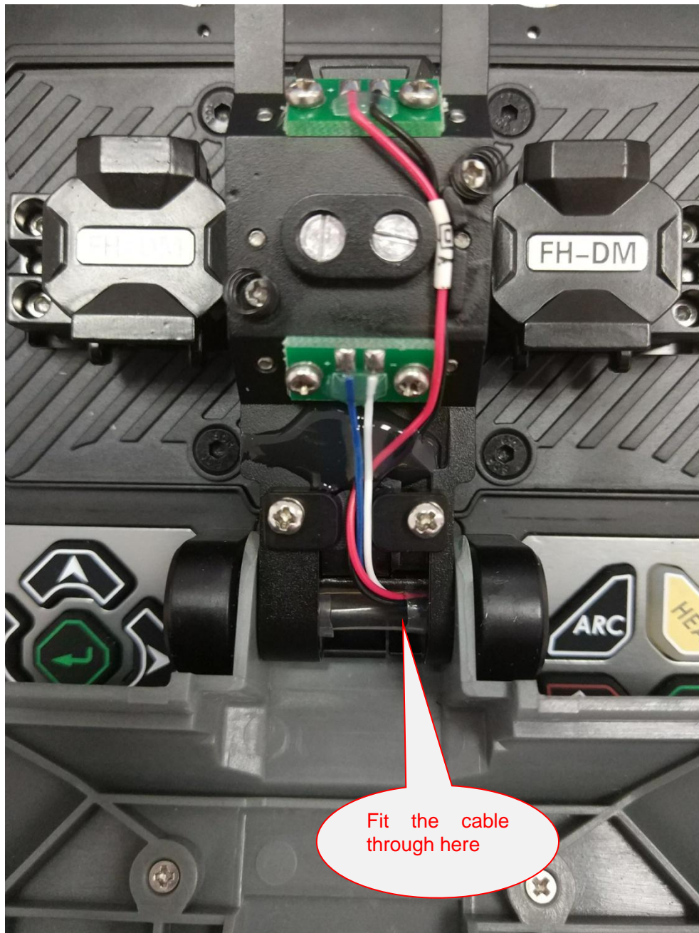
Fig.14 Installation of imaging lamp
