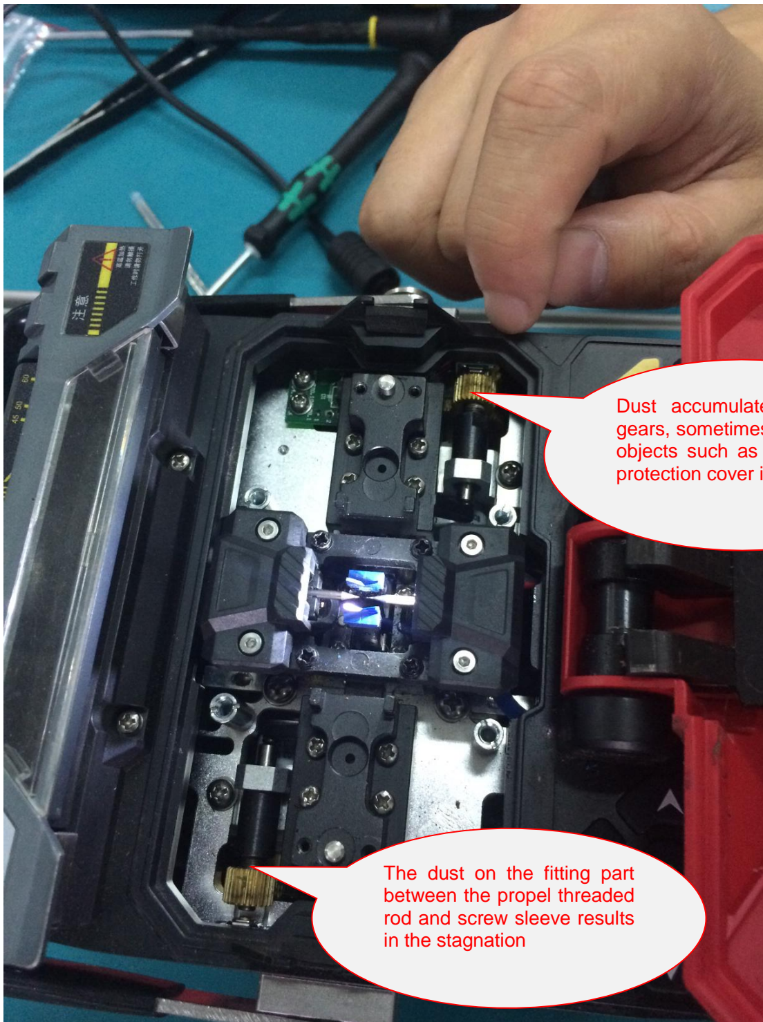
Fig.5 Cleaning of foreign objects between motor gears
