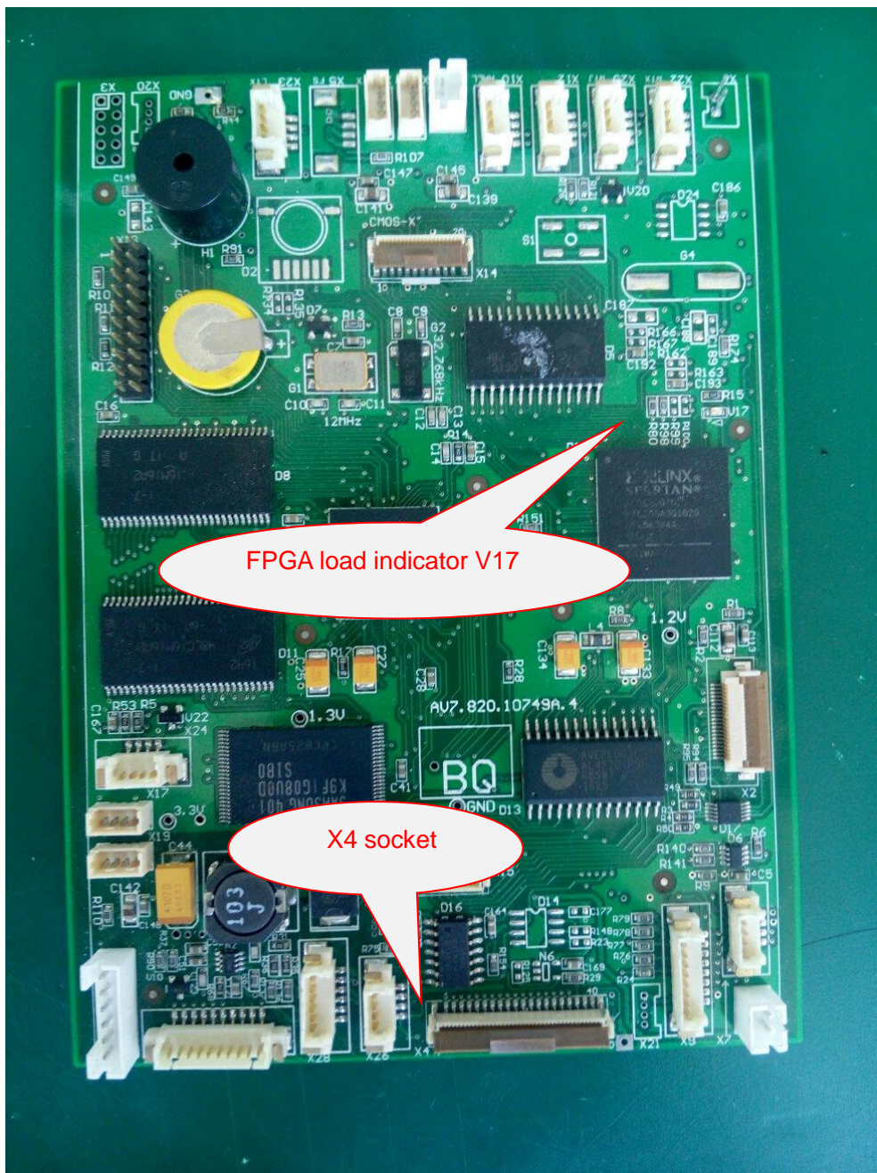
Fig.18 Main control panel
