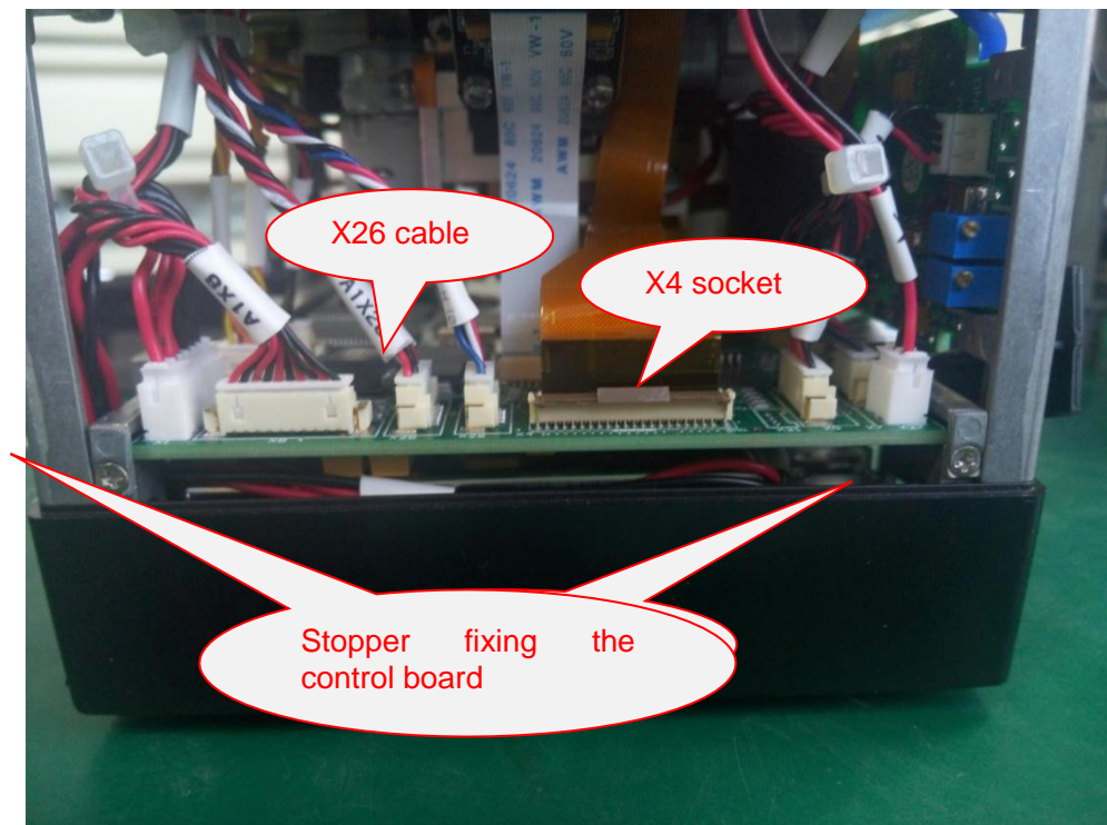
Fig.19 Stopper of main control panel
