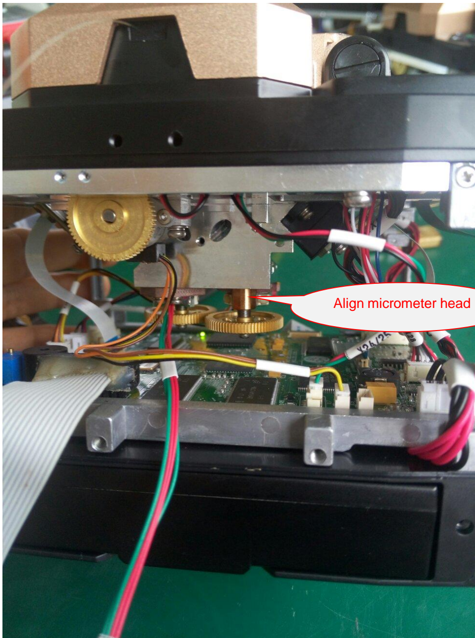
Fig.9 Align micrometer head
