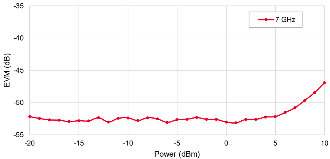
Measured EVM performance vs. power WLAN 802.11be, 320 MHz, MCS13, 300 \mu s Ch Estimation Seq Only
