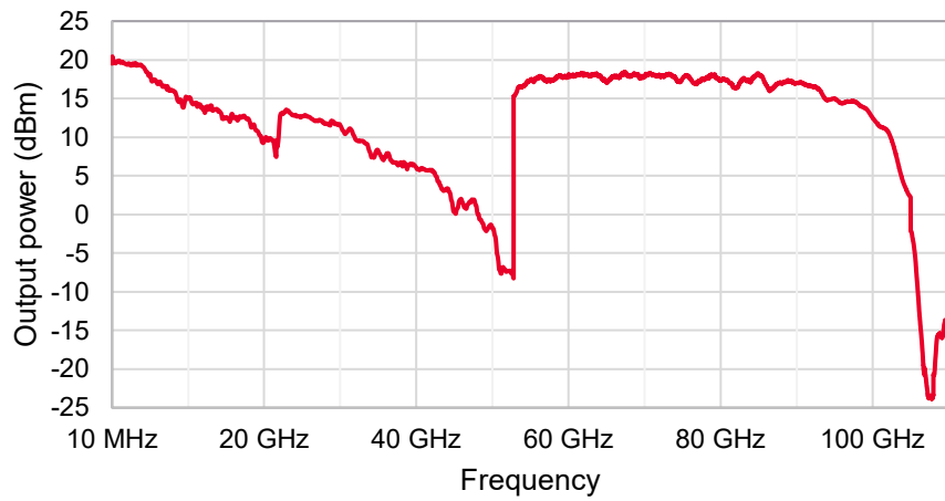
Measured maximum output power (V3080A)
